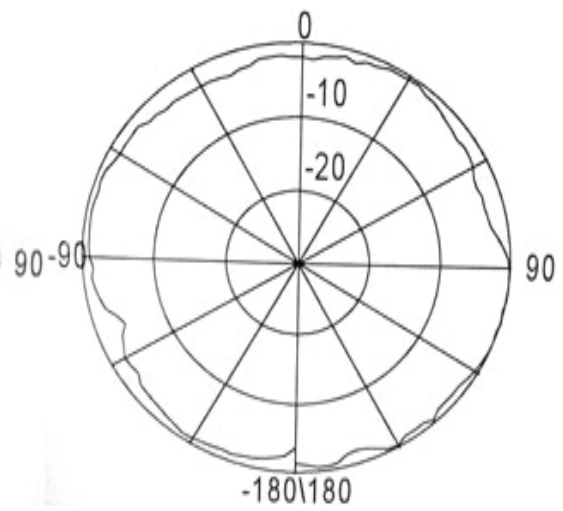
H Plane
